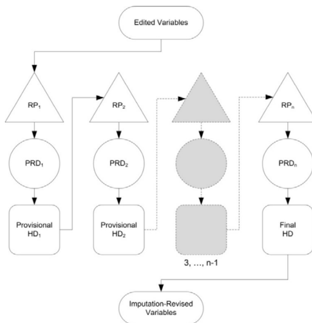
Figure 3.3 PMN Type 2: Multiple Response Propensity/Multiple Prediction
